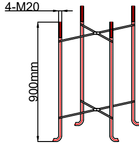
ANCHOR BOLT DETAIL
